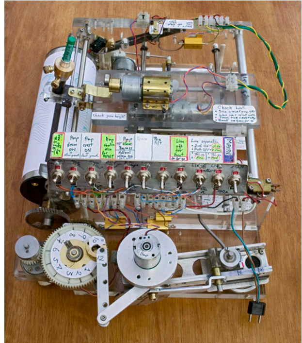
MkII Sinewave machine with 'wave break' mechanism
