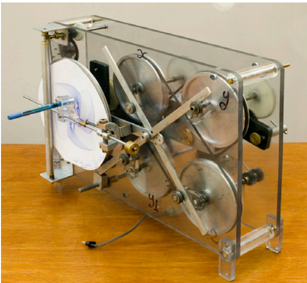
MkII Linkogram - refer also to diagram on page 13
