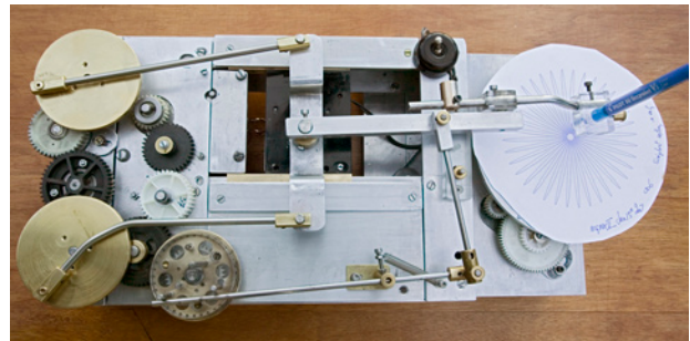
'Meccanograph' type machine with variable X axis amplitude
