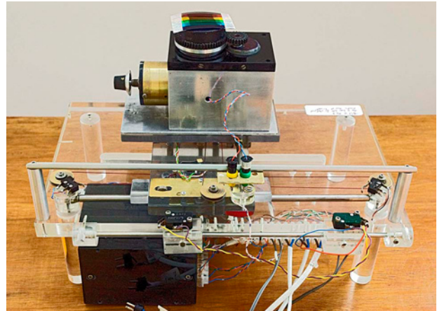
NSEW machine with rotating pen unit in place
